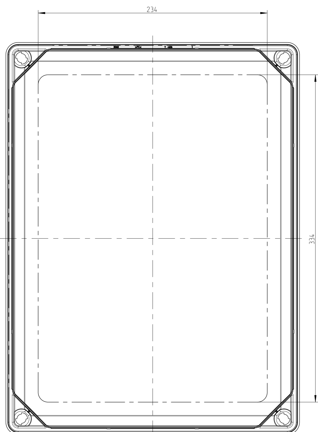
Deckel Innenansicht cover inside
